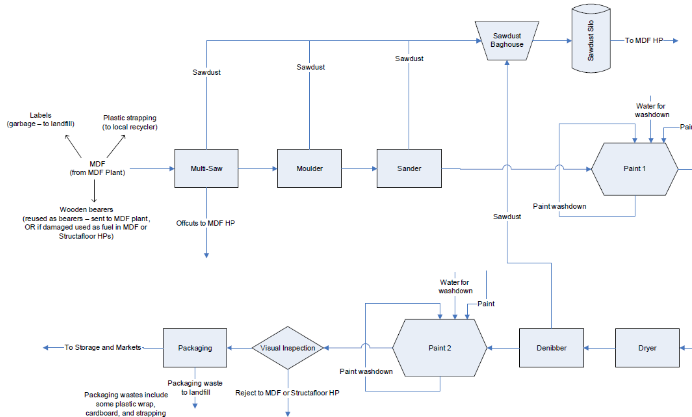
Figure 2 – Schematic Overview of the Mouldings Production Process
