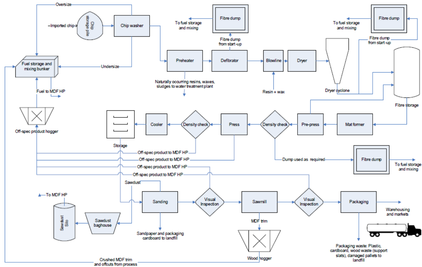
Figure 1 – Schematic Overview of the MDF Production Process
